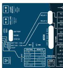
KNECT Endpoint (KEP-200)
